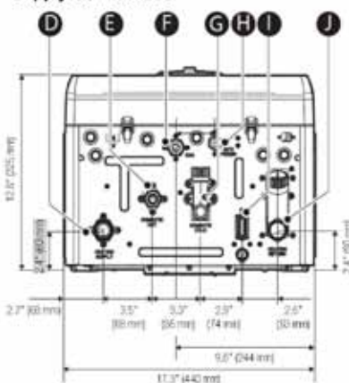
Supply Connections
