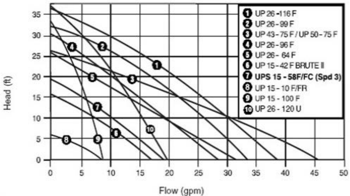
UP / UPS Series Pump Curve
